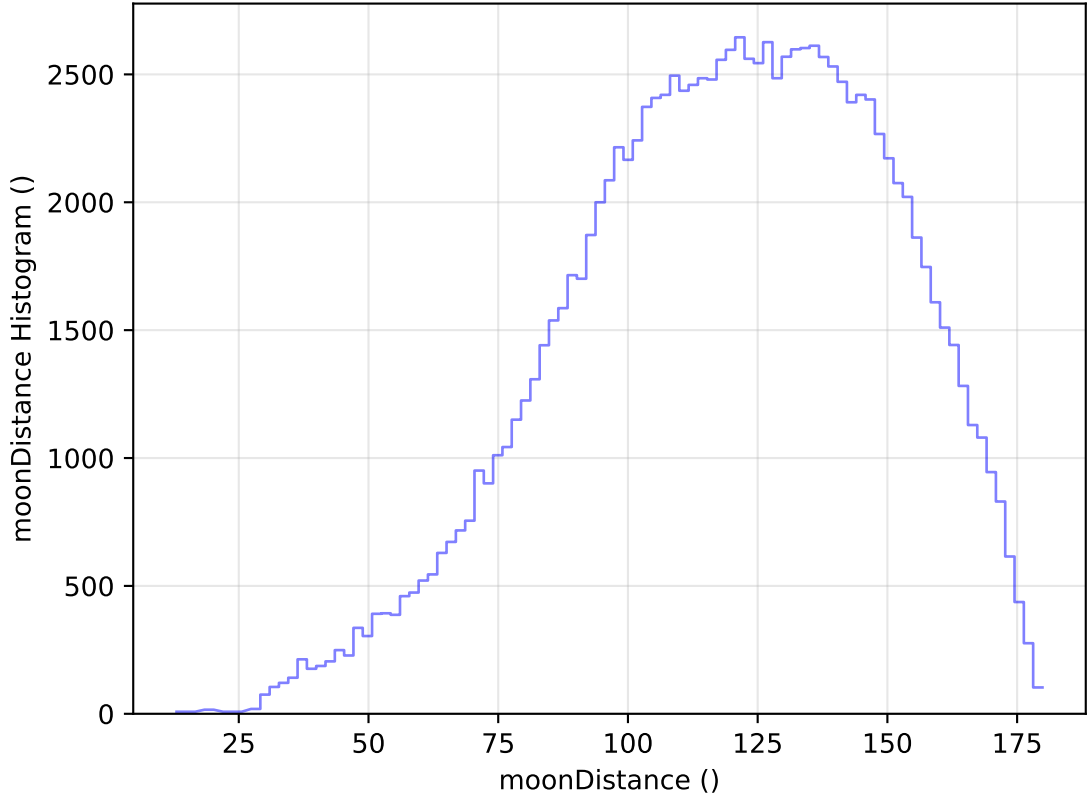
too_elab_heavy_r32_d3_ugrizy_v3.4_10yrs All sky u band: moonDistance Histogram
