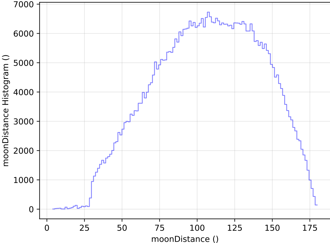
too_elab_heavy_r32_d3_ugrizy_v3.4_10yrs All sky r band: moonDistance Histogram
