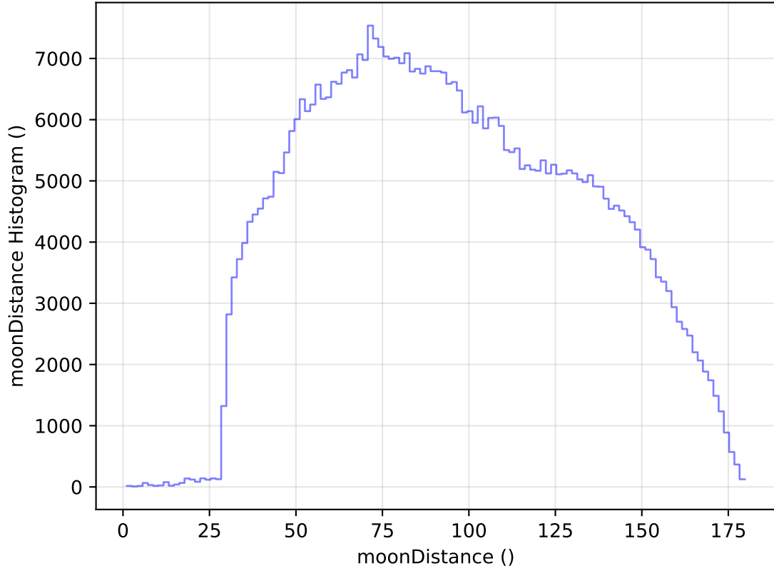
too_elab_heavy_r32_d3_ugrizy_v3.4_10yrs All sky i band: moonDistance Histogram
