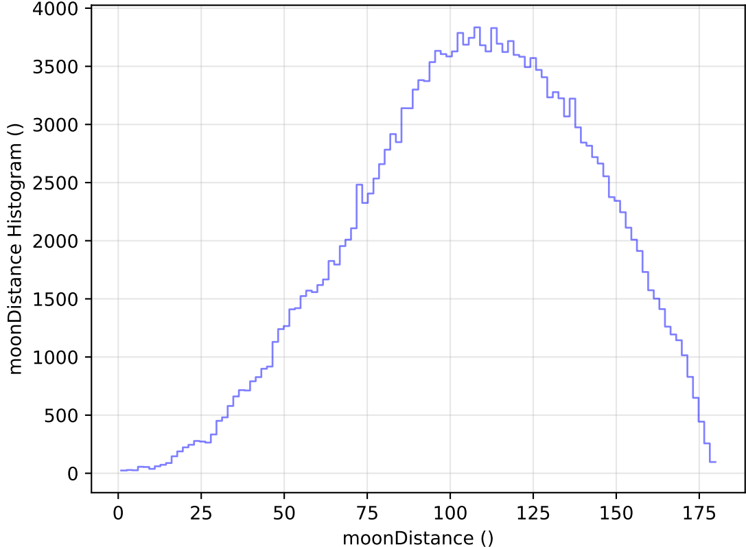
too_elab_heavy_r32_d3_ugrizy_v3.4_10yrs All sky g band: moonDistance Histogram
