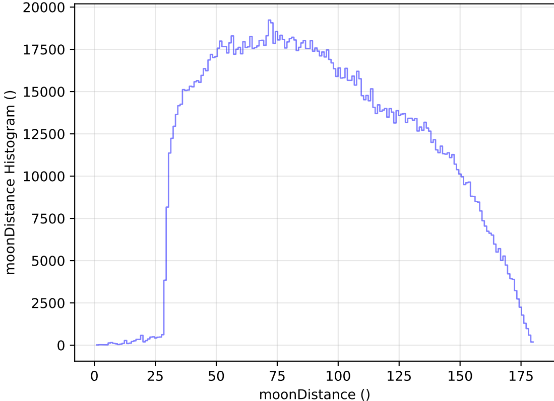
too_elab_heavy_r32_d3_ugrizy_v3.4_10yrs All sky all bands: moonDistance Histogram
