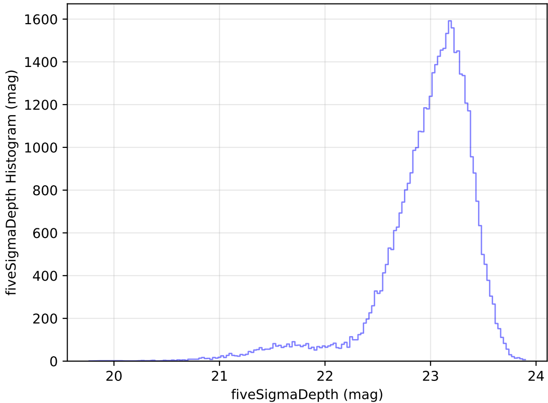
too_elab_heavy_r32_d3_ugrizy_v3.4_10yrs Yr 1 z band: fiveSigmaDepth Histogram
