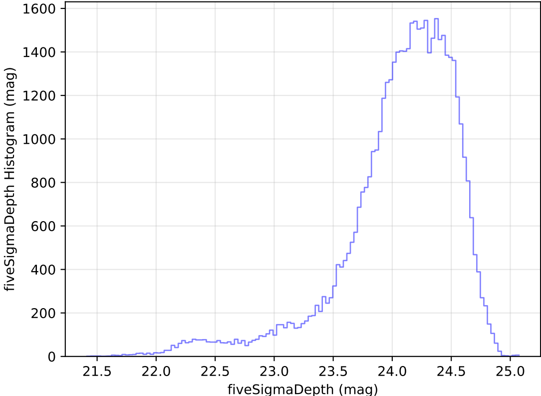
too_elab_heavy_r32_d3_ugrizy_v3.4_10yrs Yr 1 r band: fiveSigmaDepth Histogram
