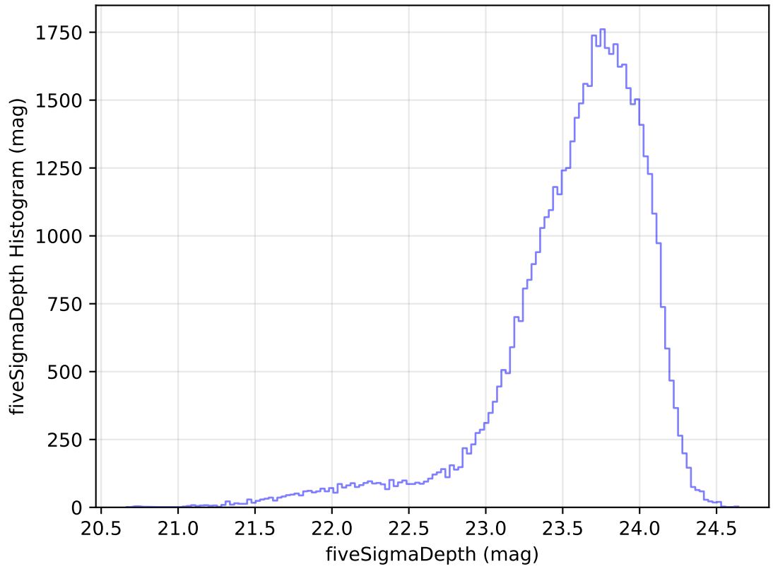
too_elab_heavy_r32_d3_ugrizy_v3.4_10yrs Yr 1 i band: fiveSigmaDepth Histogram
