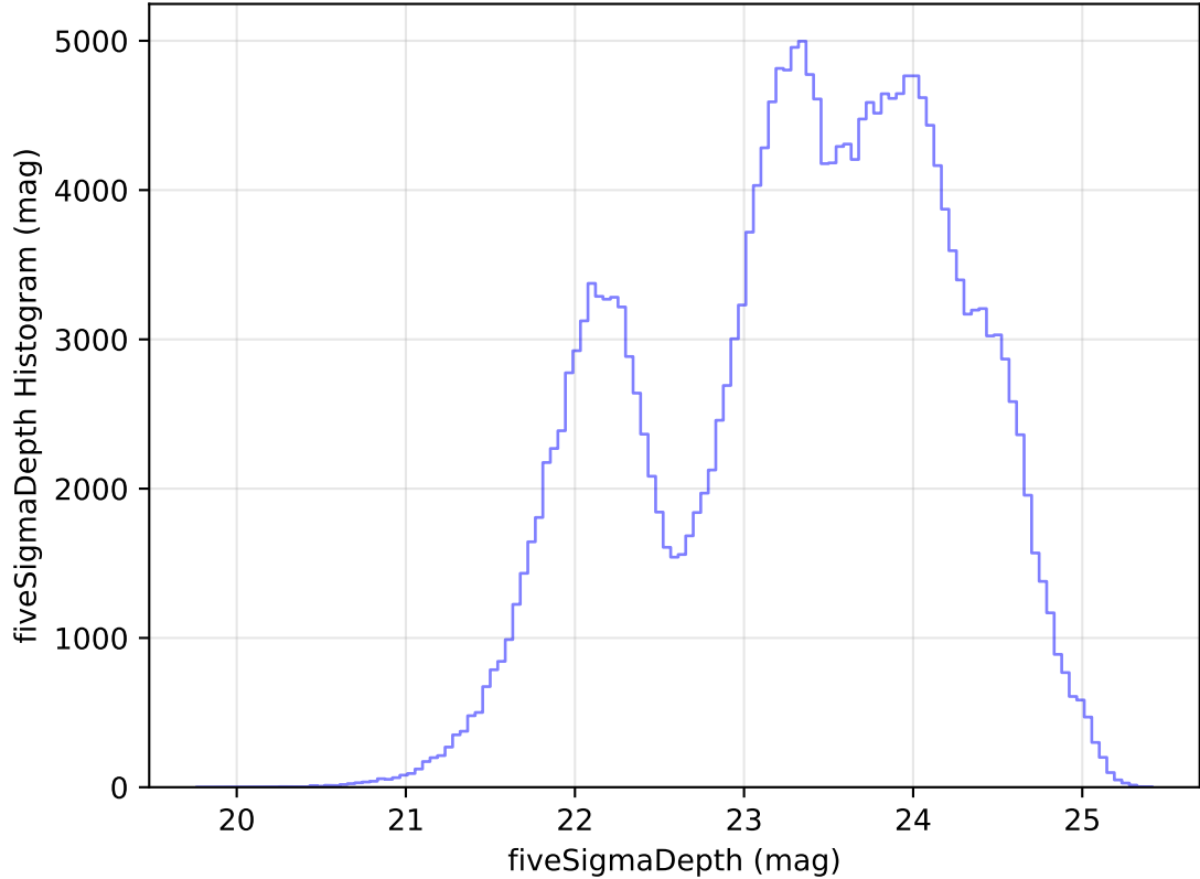
too_elab_heavy_r32_d3_ugrizy_v3.4_10yrs Yr 1 all bands: fiveSigmaDepth Histogram
