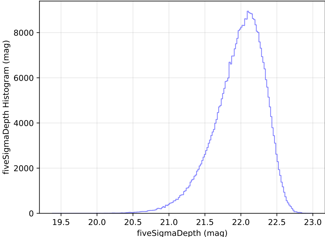
too_elab_heavy_r32_d3_ugrizy_v3.4_10yrs WFD y band: fiveSigmaDepth Histogram
