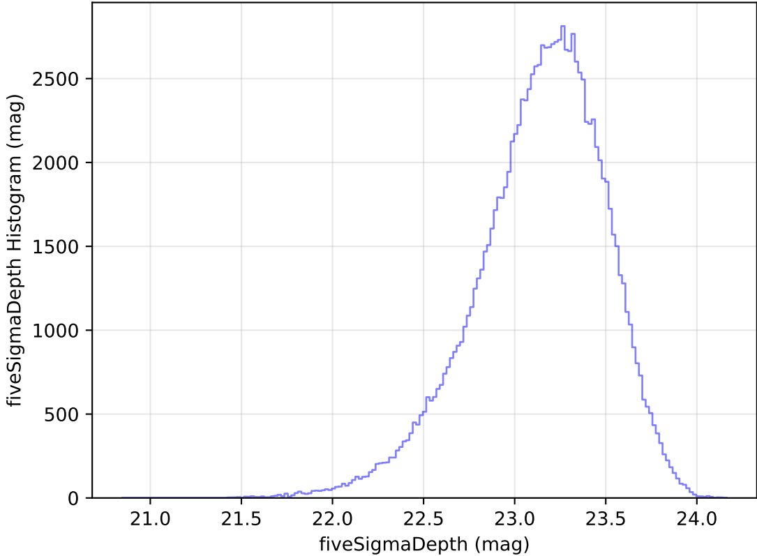
too_elab_heavy_r32_d3_ugrizy_v3.4_10yrs WFD u band: fiveSigmaDepth Histogram
