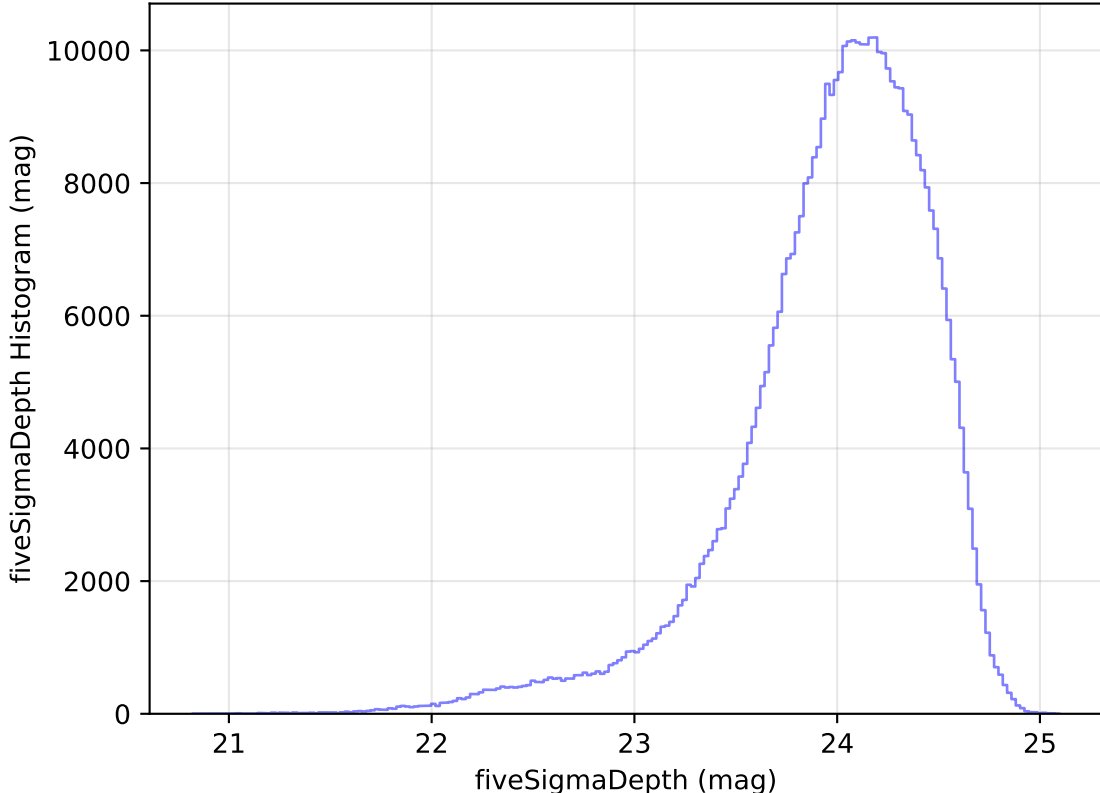
too_elab_heavy_r32_d3_ugrizy_v3.4_10yrs WFD r band: fiveSigmaDepth Histogram
