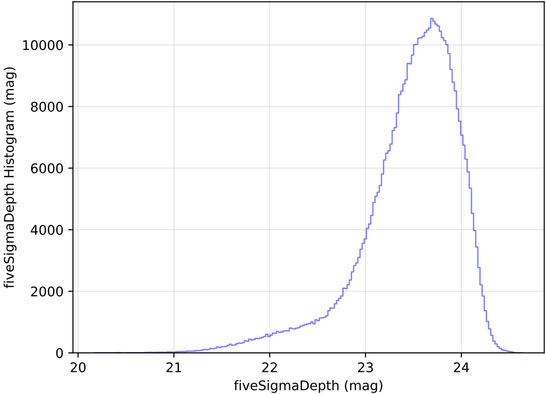
too_elab_heavy_r32_d3_ugrizy_v3.4_10yrs WFD i band: fiveSigmaDepth Histogram
