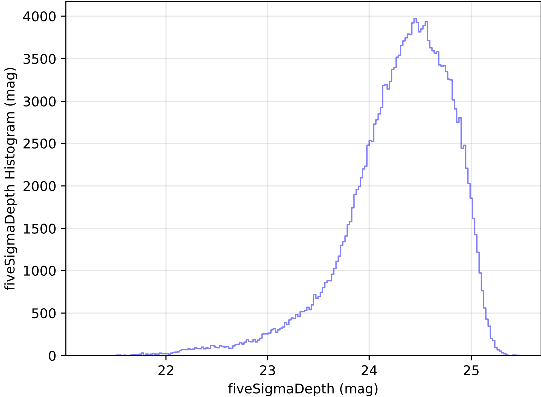
too_elab_heavy_r32_d3_ugrizy_v3.4_10yrs WFD g band: fiveSigmaDepth Histogram
