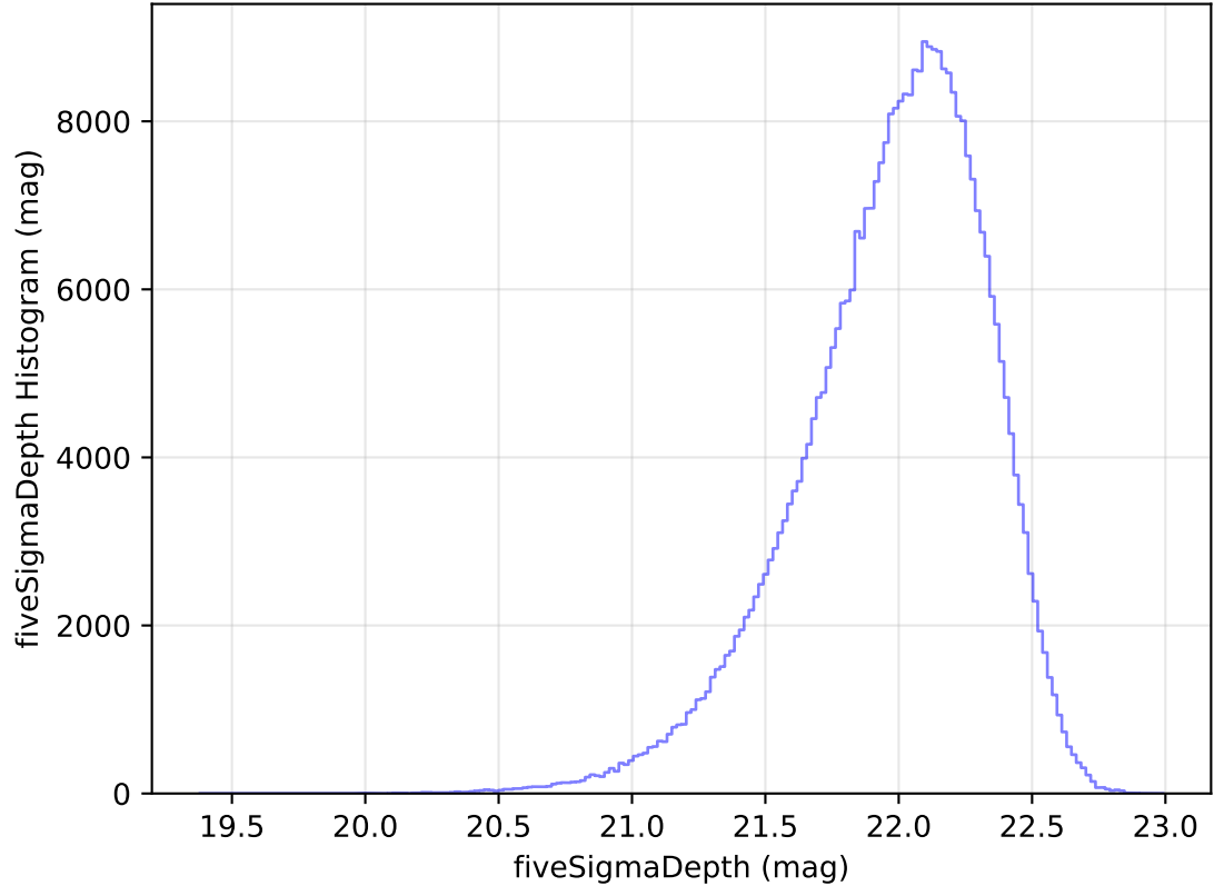
too_elab_heavy_r32_d3_ugrizy_v3.4_10yrs All sky y band: fiveSigmaDepth Histogram
