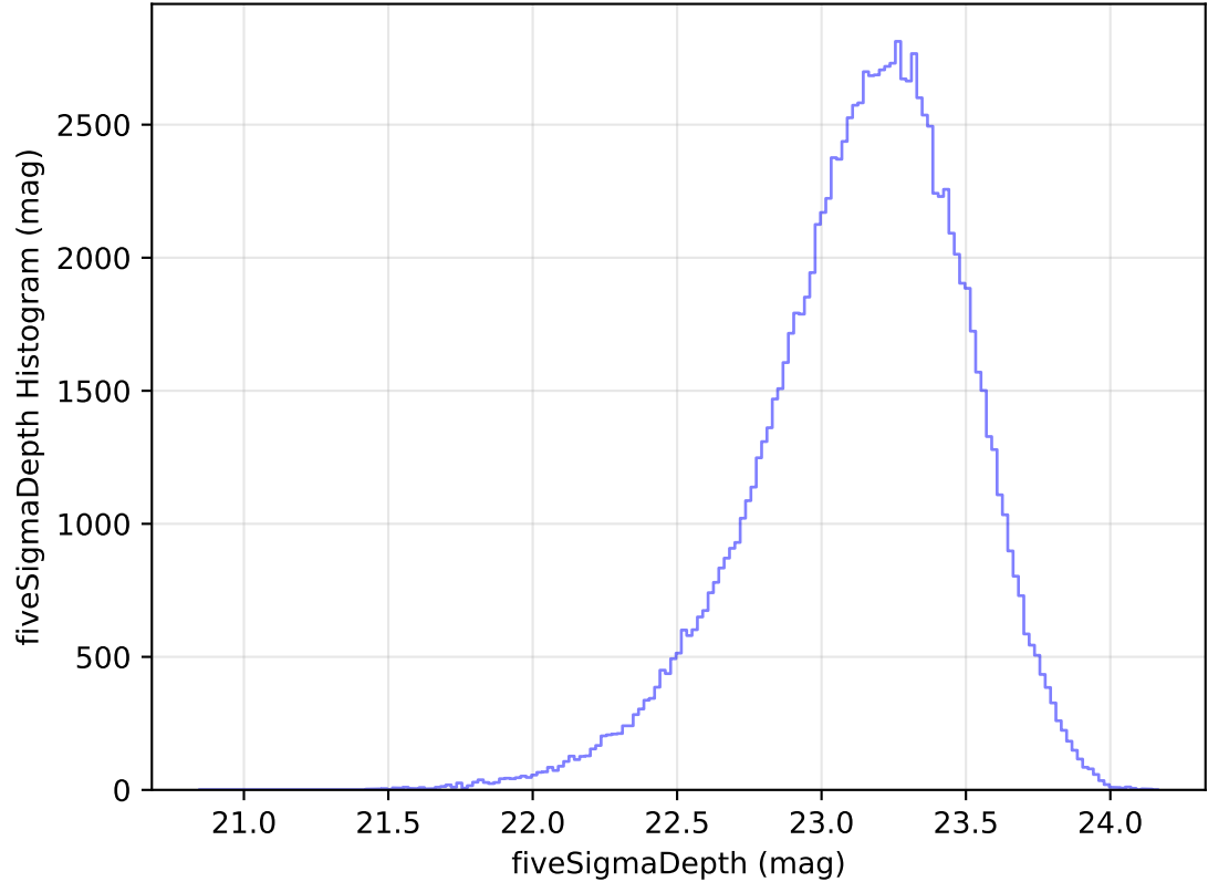
too_elab_heavy_r32_d3_ugrizy_v3.4_10yrs All sky u band: fiveSigmaDepth Histogram
