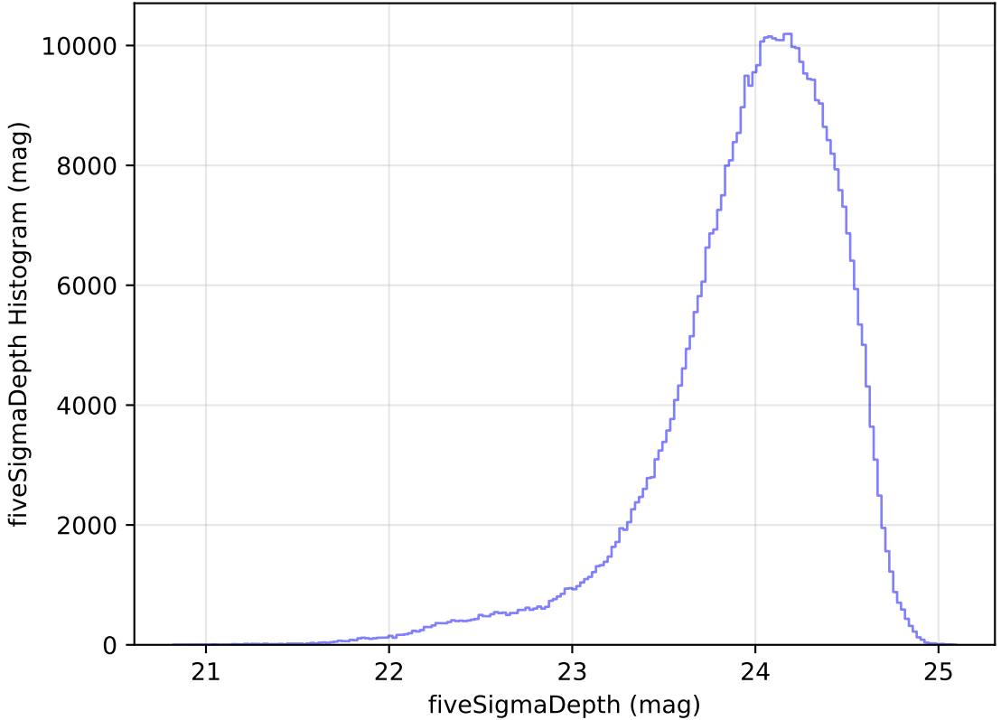
too_elab_heavy_r32_d3_ugrizy_v3.4_10yrs All sky r band: fiveSigmaDepth Histogram
