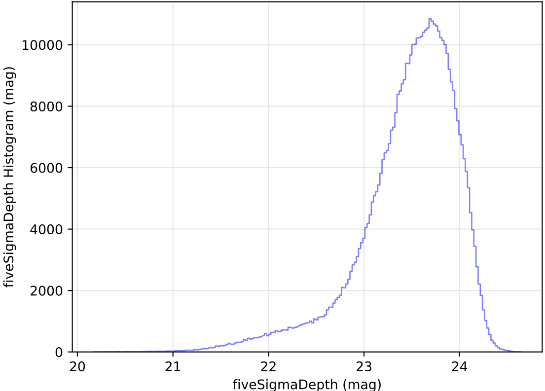
too_elab_heavy_r32_d3_ugrizy_v3.4_10yrs All sky i band: fiveSigmaDepth Histogram
