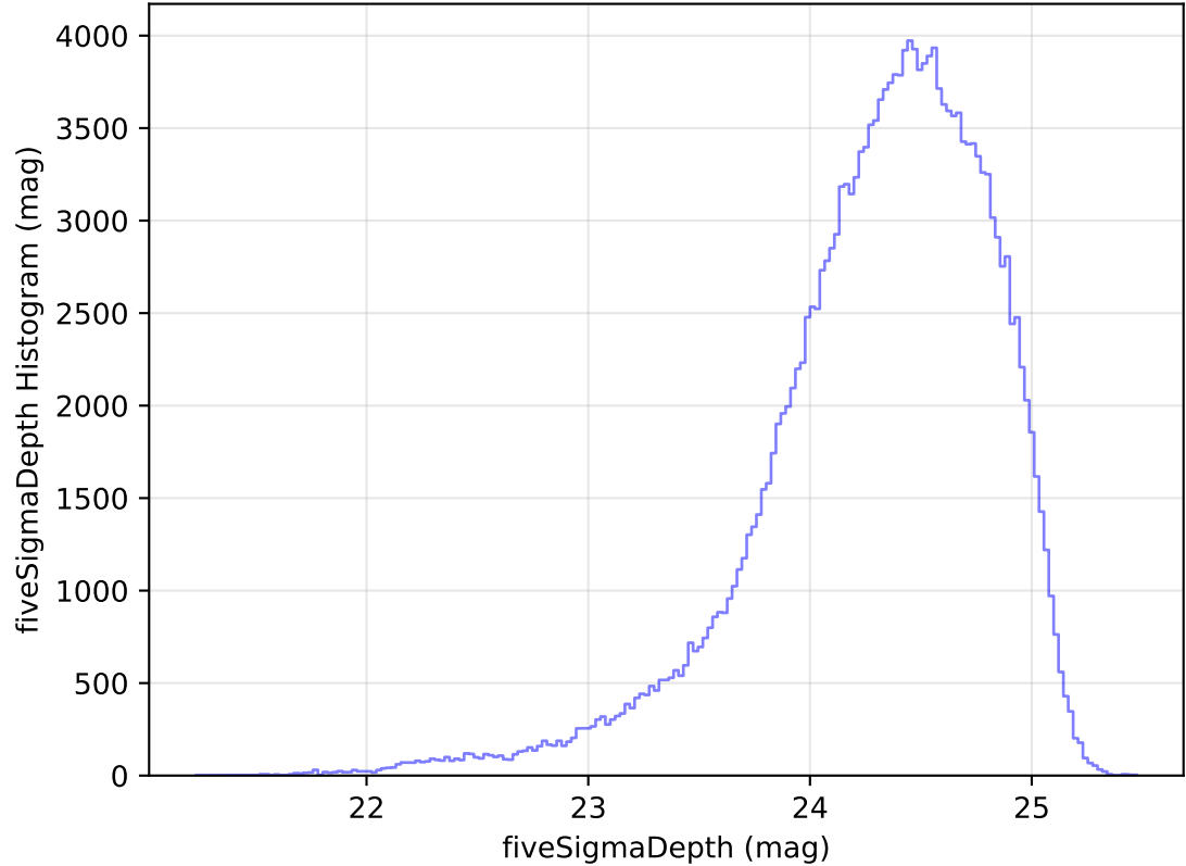
too_elab_heavy_r32_d3_ugrizy_v3.4_10yrs All sky g band: fiveSigmaDepth Histogram
