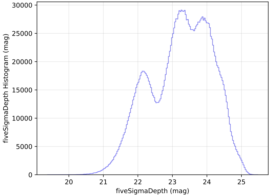
too_elab_heavy_r32_d3_ugrizy_v3.4_10yrs All sky all bands: fiveSigmaDepth Histogram
