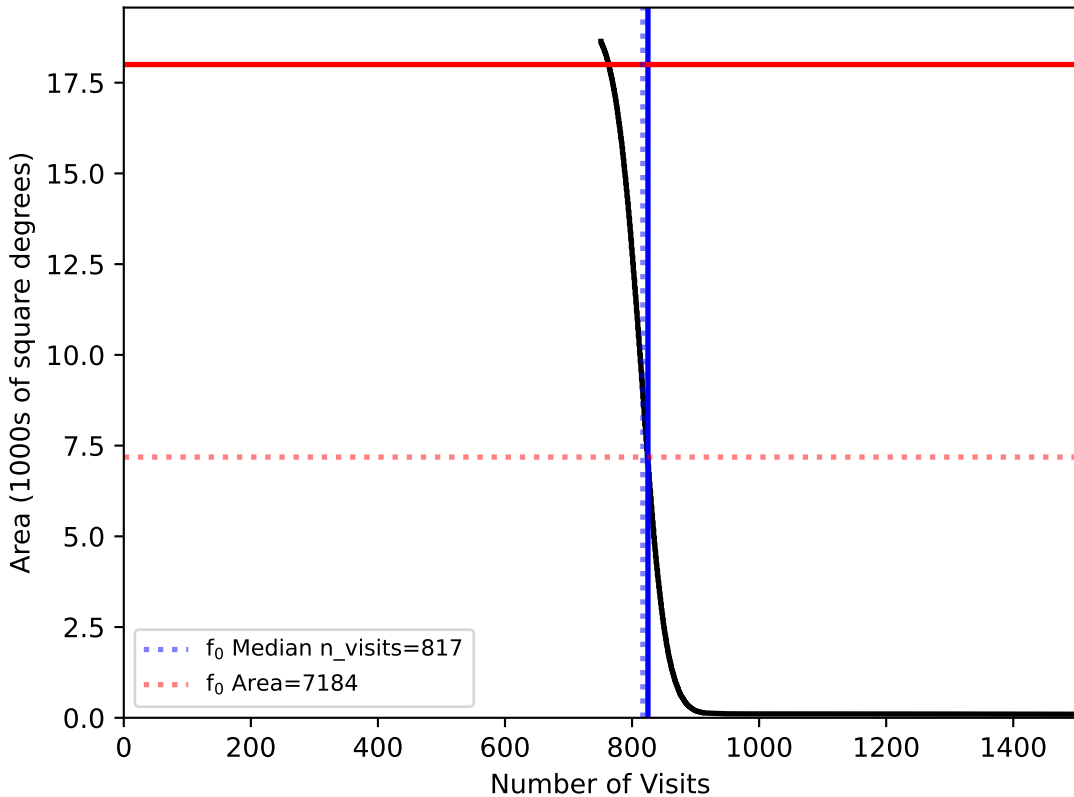
too_elab_heavy_r32_d3_ugrizy_v3.4_10yrs WFD: f0
