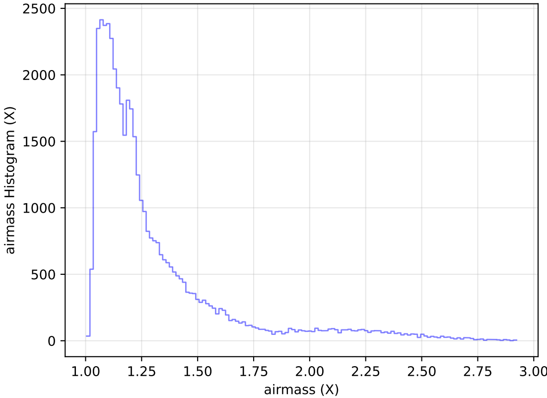
too_elab_heavy_r32_d3_ugrizy_v3.4_10yrs Yr 1 z band: airmass Histogram
