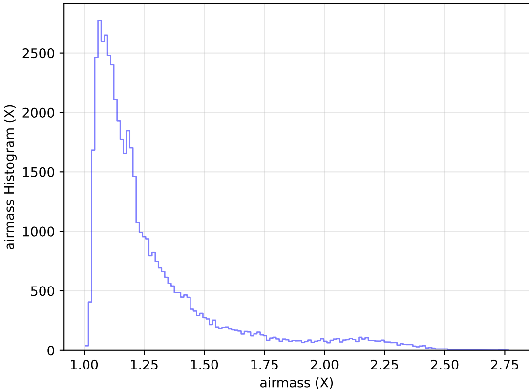
too_elab_heavy_r32_d3_ugrizy_v3.4_10yrs Yr 1 r band: airmass Histogram
