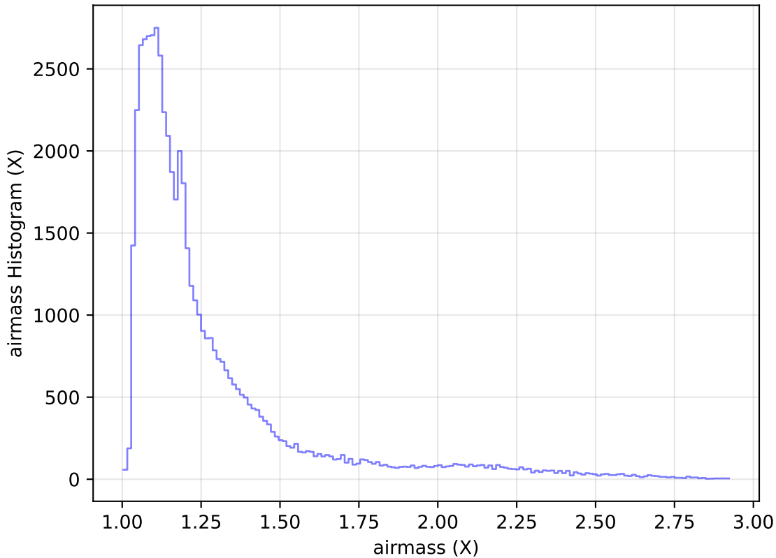
too_elab_heavy_r32_d3_ugrizy_v3.4_10yrs Yr 1 i band: airmass Histogram
