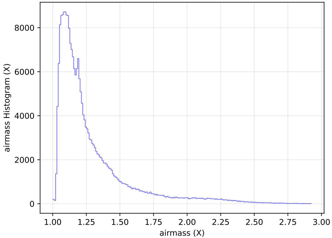
too_elab_heavy_r32_d3_ugrizy_v3.4_10yrs Yr 1 all bands: airmass Histogram
