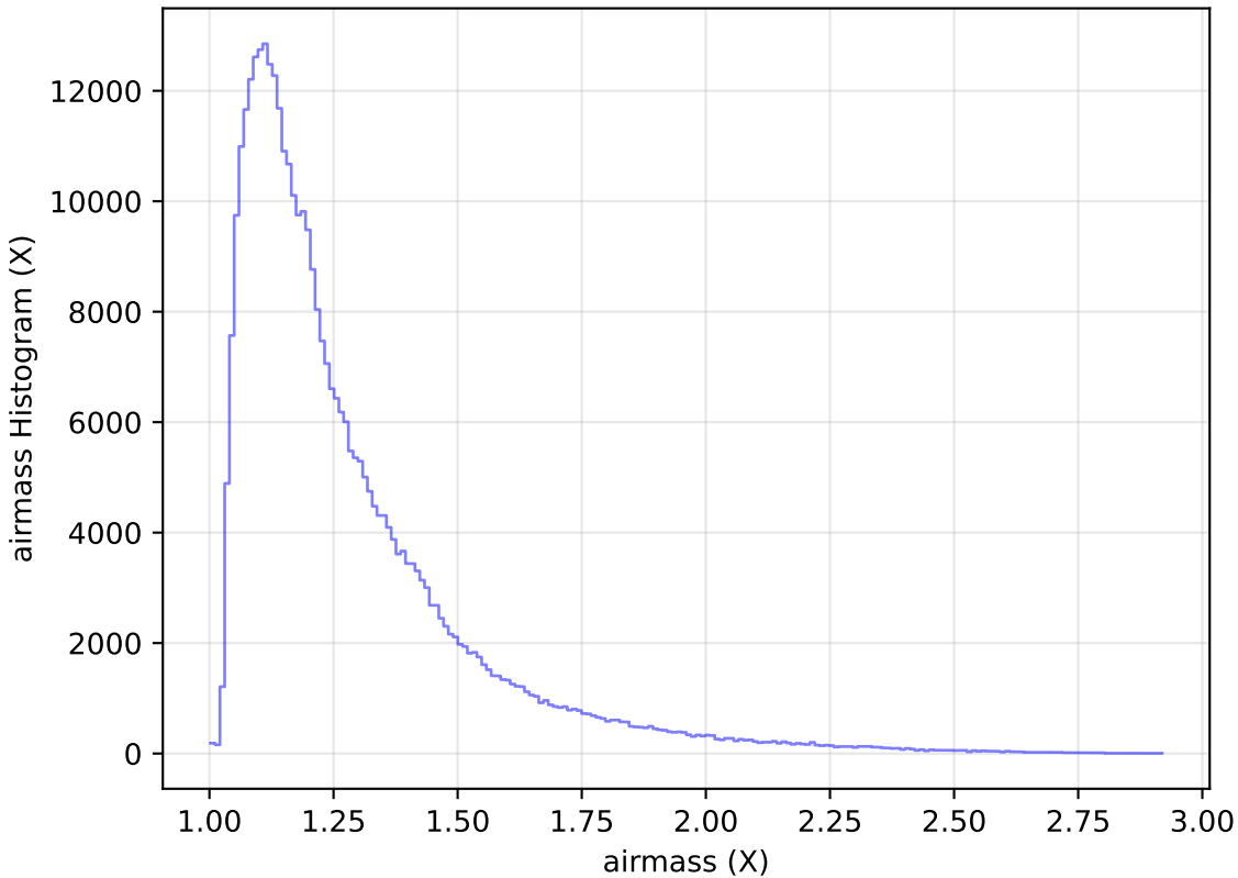
too_elab_heavy_r32_d3_ugrizy_v3.4_10yrs WFD y band: airmass Histogram
