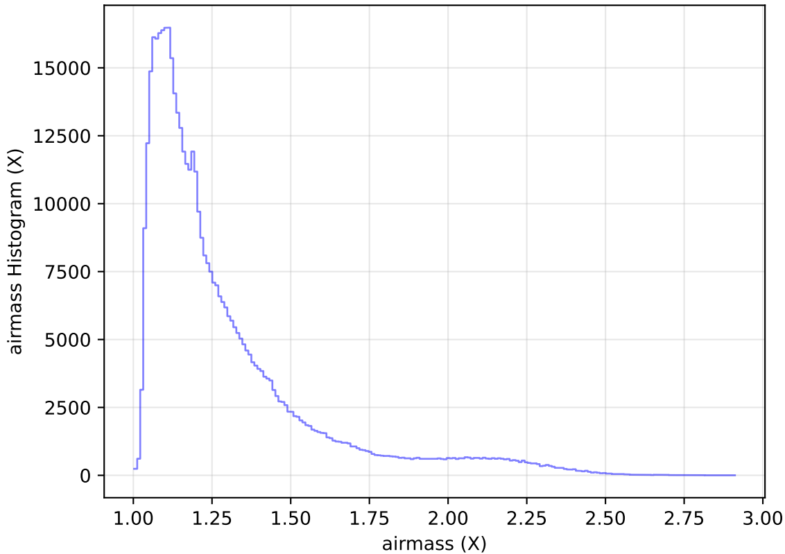
too_elab_heavy_r32_d3_ugrizy_v3.4_10yrs WFD r band: airmass Histogram
