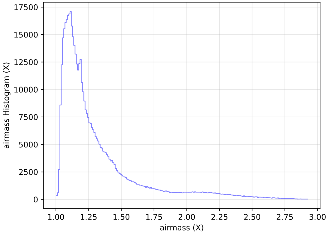
too_elab_heavy_r32_d3_ugrizy_v3.4_10yrs WFD i band: airmass Histogram
