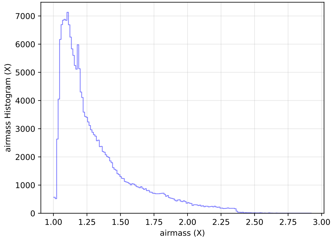
too_elab_heavy_r32_d3_ugrizy_v3.4_10yrs WFD g band: airmass Histogram
