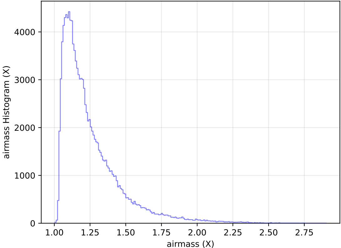
too_elab_heavy_r32_d3_ugrizy_v3.4_10yrs All sky u band: airmass Histogram
