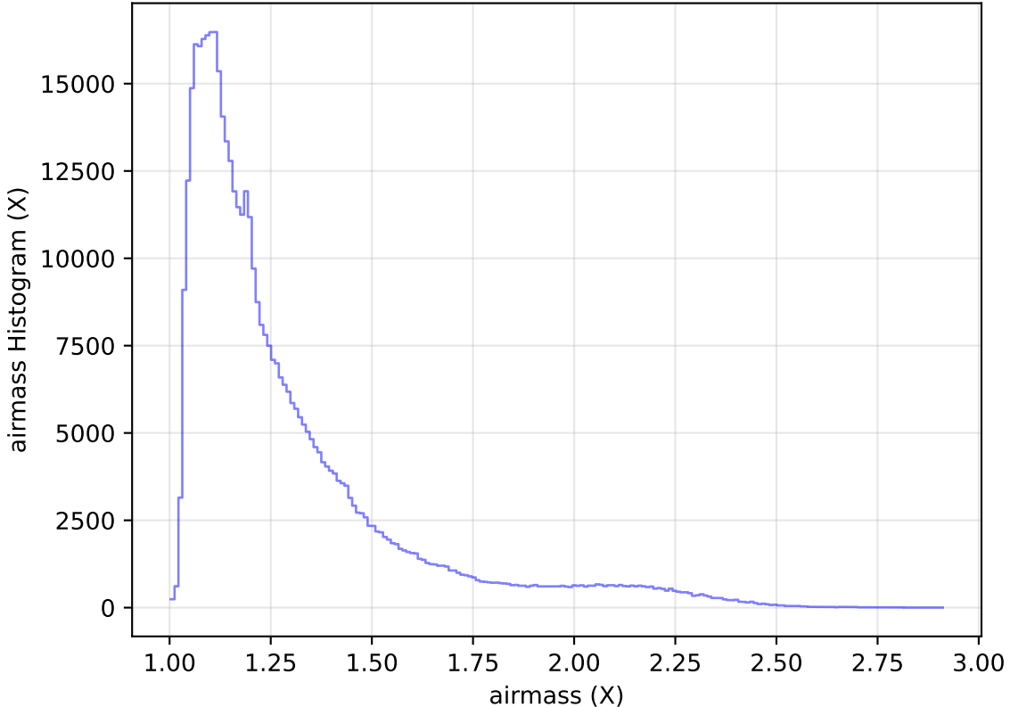
too_elab_heavy_r32_d3_ugrizy_v3.4_10yrs All sky r band: airmass Histogram
