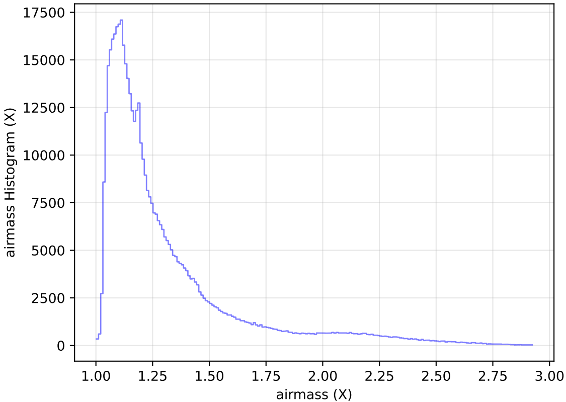
too_elab_heavy_r32_d3_ugrizy_v3.4_10yrs All sky i band: airmass Histogram
