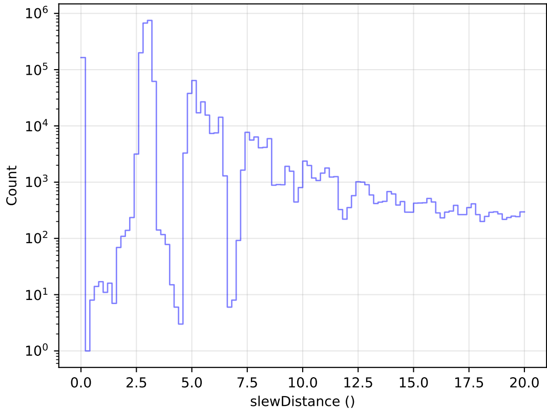
too_elab_heavy_r32_d3_ugrizy_v3.4_10yrs All visits: Zoom Slew Distance Histogram
