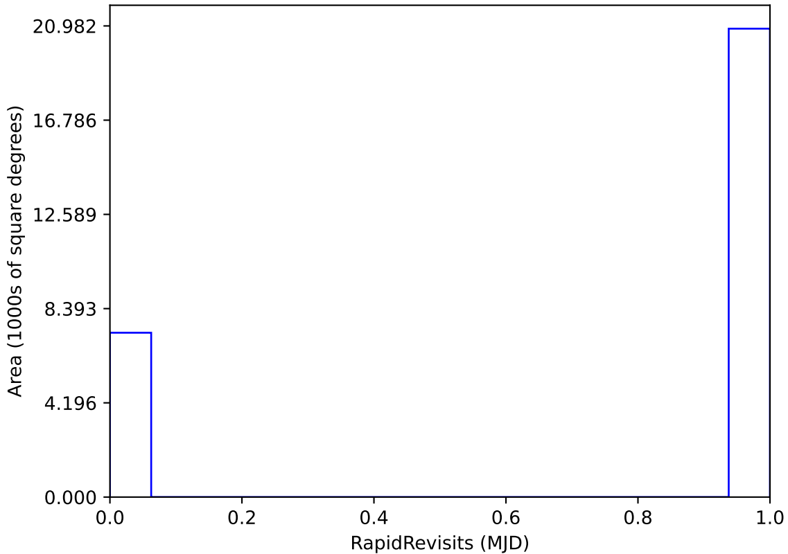
too_elab_heavy_r32_d3_ugrizy_v3.4_10yrs All sky: RapidRevisits
