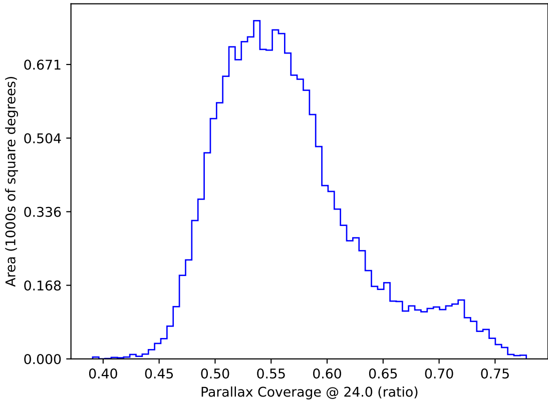
too_elab_heavy_r32_d3_ugrizy_v3.4_10yrs WFD: Parallax Coverage @ 24.0
