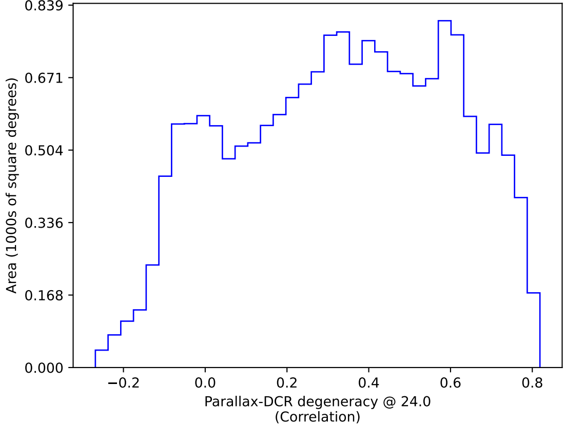
too_elab_heavy_r32_d3_ugrizy_v3.4_10yrs WFD: Parallax-DCR degeneracy @ 24.0
