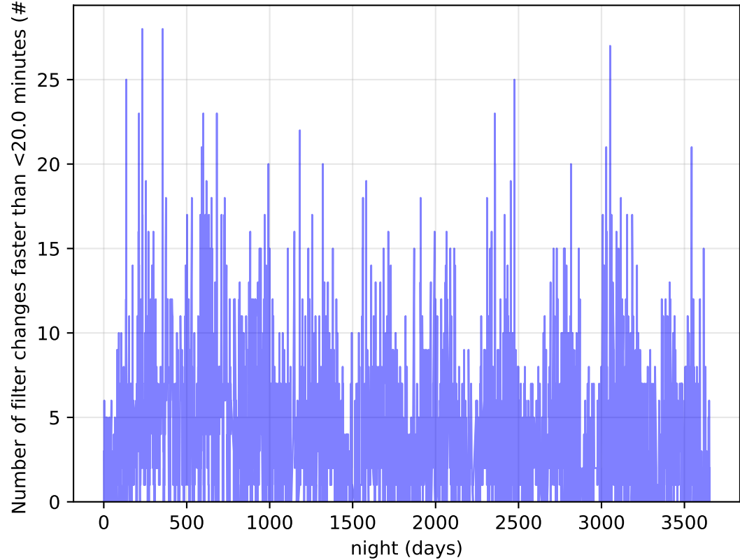
too_elab_heavy_r32_d3_ugrizy_v3.4_10yrs Per Night: Number of filter changes faster than <20.0 minutes
