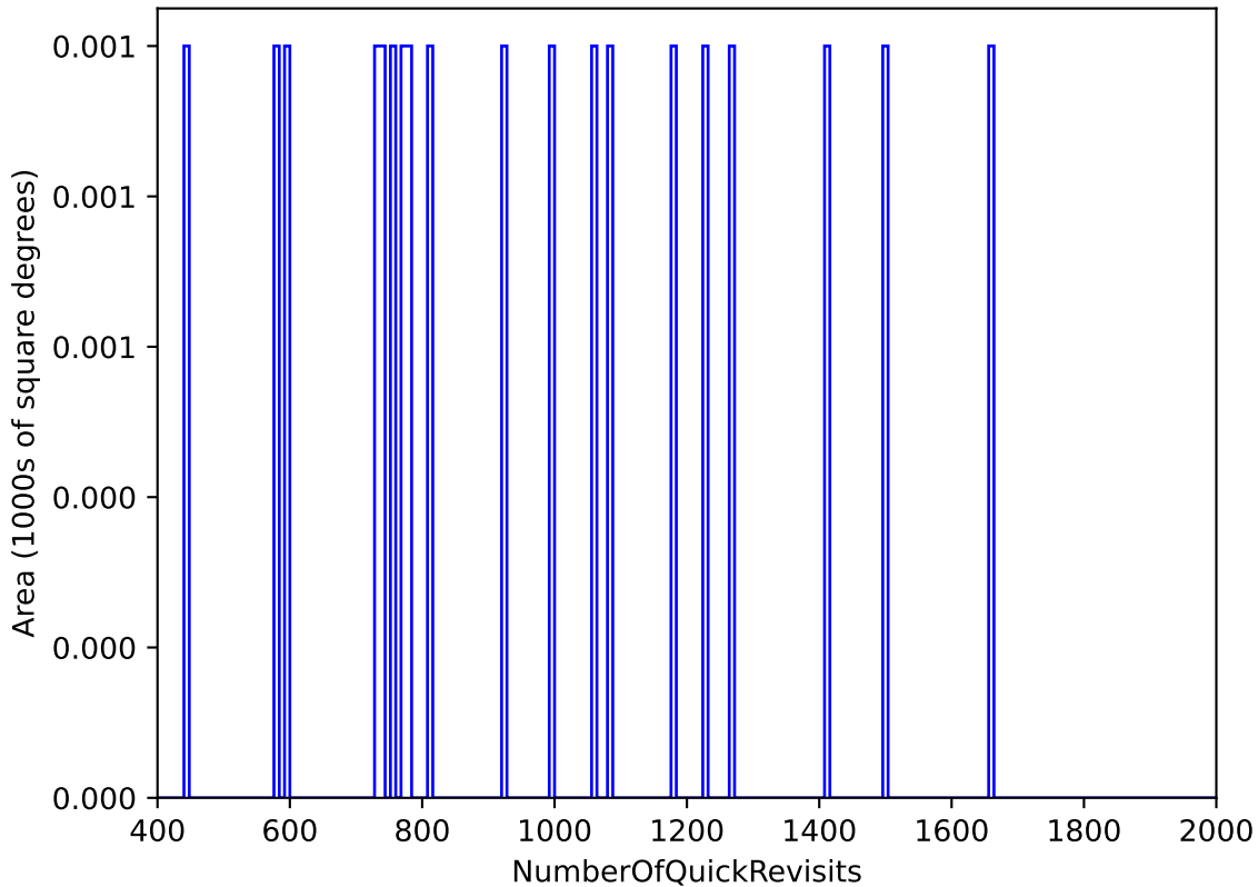
too_elab_heavy_r32_d3_ugrizy_v3.4_10yrs All sky: NumberOfQuickRevisits
