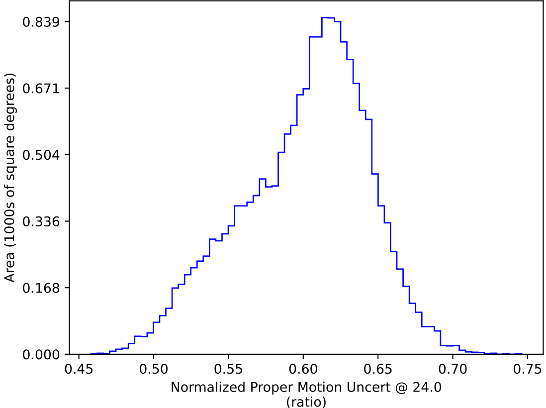
too_elab_heavy_r32_d3_ugrizy_v3.4_10yrs WFD: Normalized Proper Motion Uncert @ 24.0
