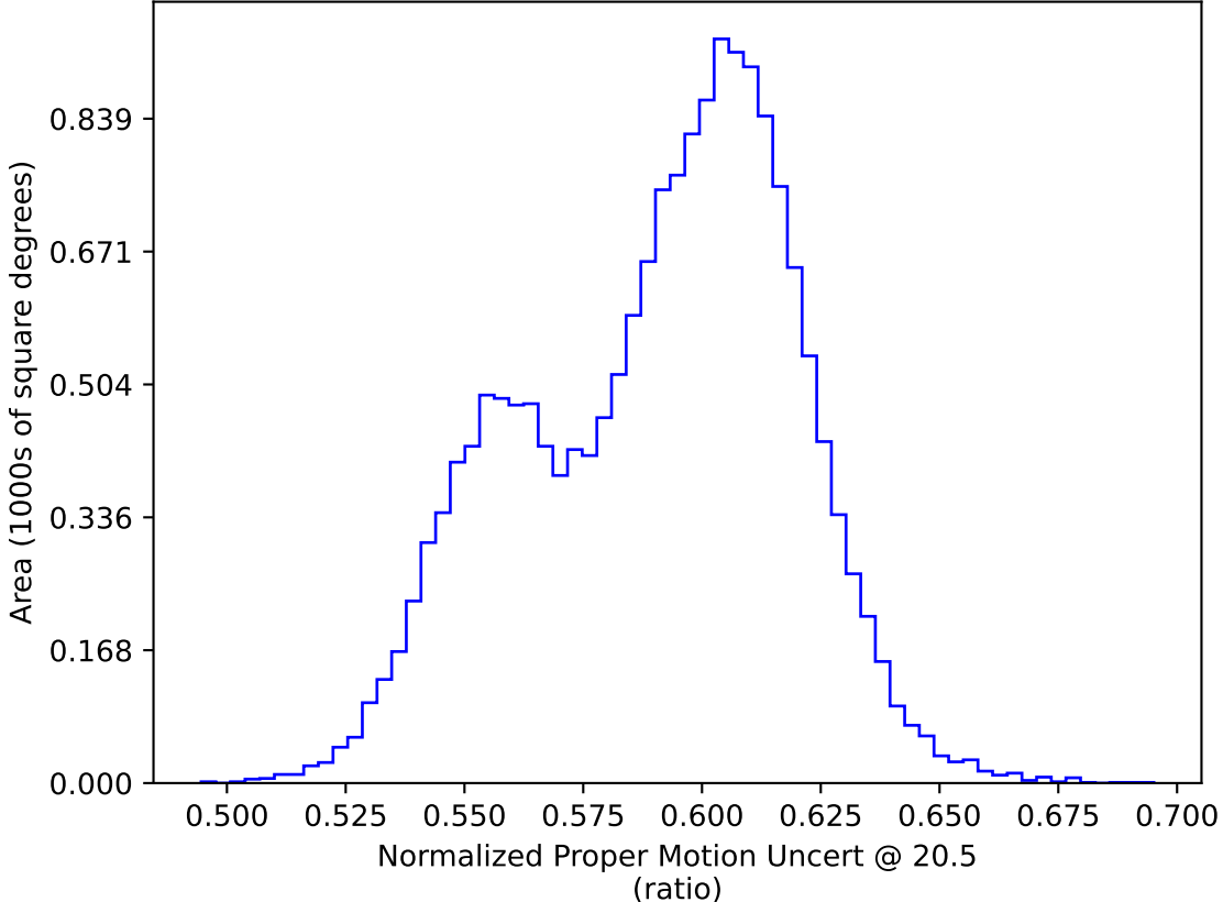
too_elab_heavy_r32_d3_ugrizy_v3.4_10yrs WFD: Normalized Proper Motion Uncert @ 20.5
