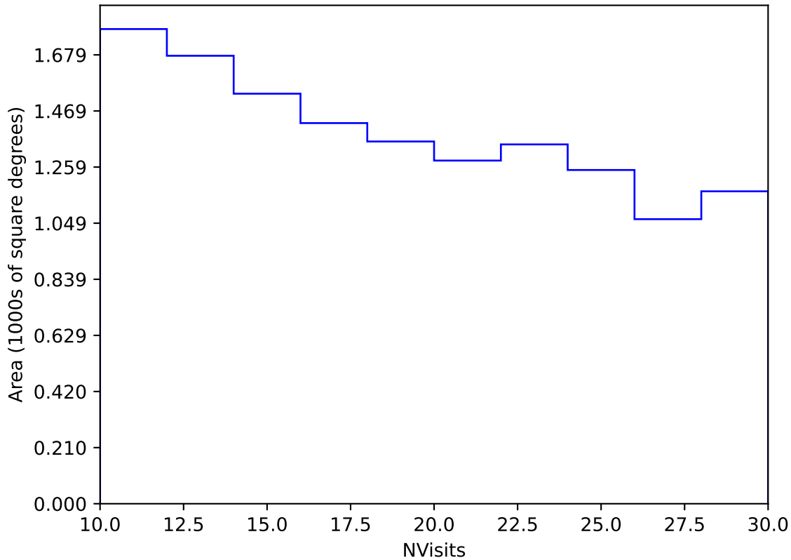
too_elab_heavy_r32_d3_ugrizy_v3.4_10yrs Yr 3-4 y band: NVisits
