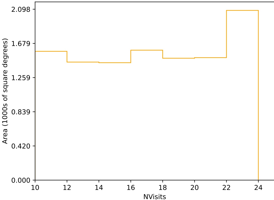
too_elab_heavy_r32_d3_ugrizy_v3.4_10yrs Yr 3-4 r band: NVisits
