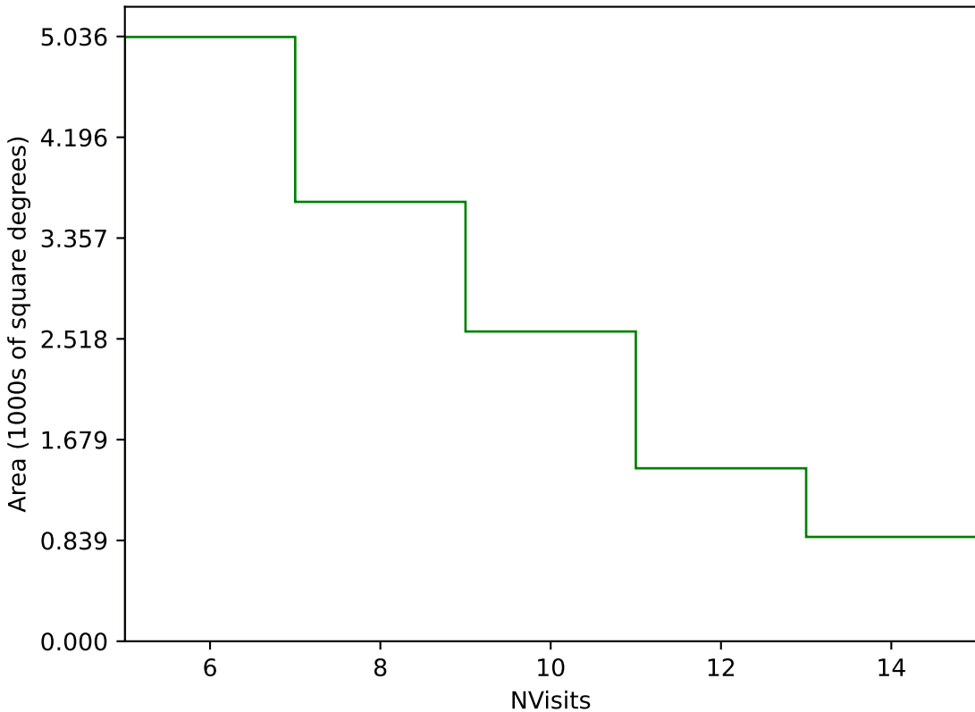
too_elab_heavy_r32_d3_ugrizy_v3.4_10yrs Yr 3-4 g band: NVisits
