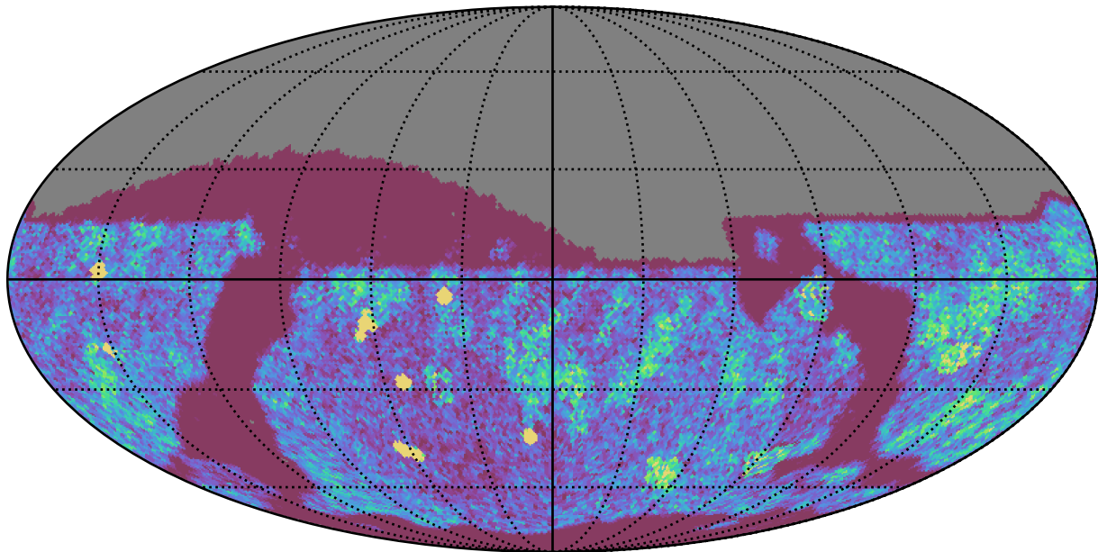
too_elab_heavy_r32_d3_ugrizy_v3.4_10yrs Yr 1 z band: NVisits
