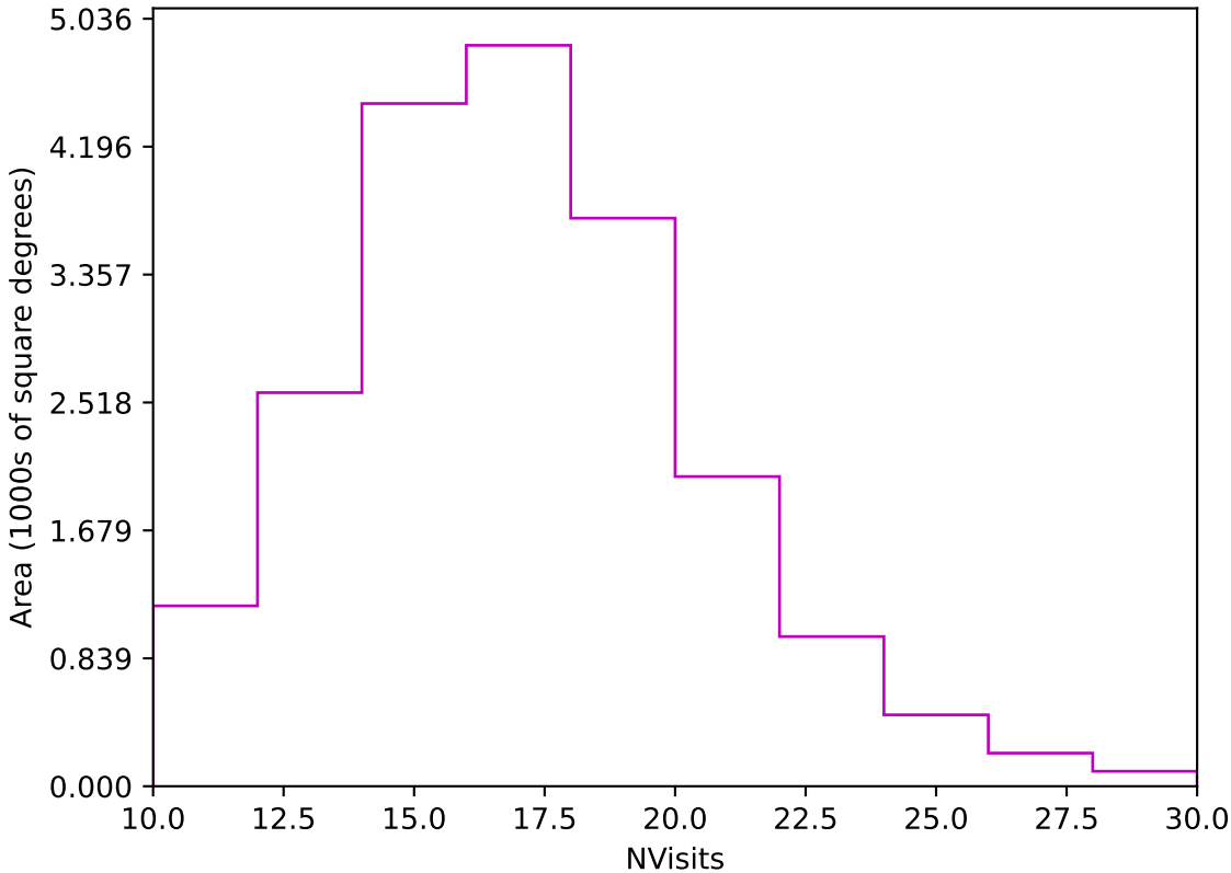
too_elab_heavy_r32_d3_ugrizy_v3.4_10yrs Yr 1 z band: NVisits
