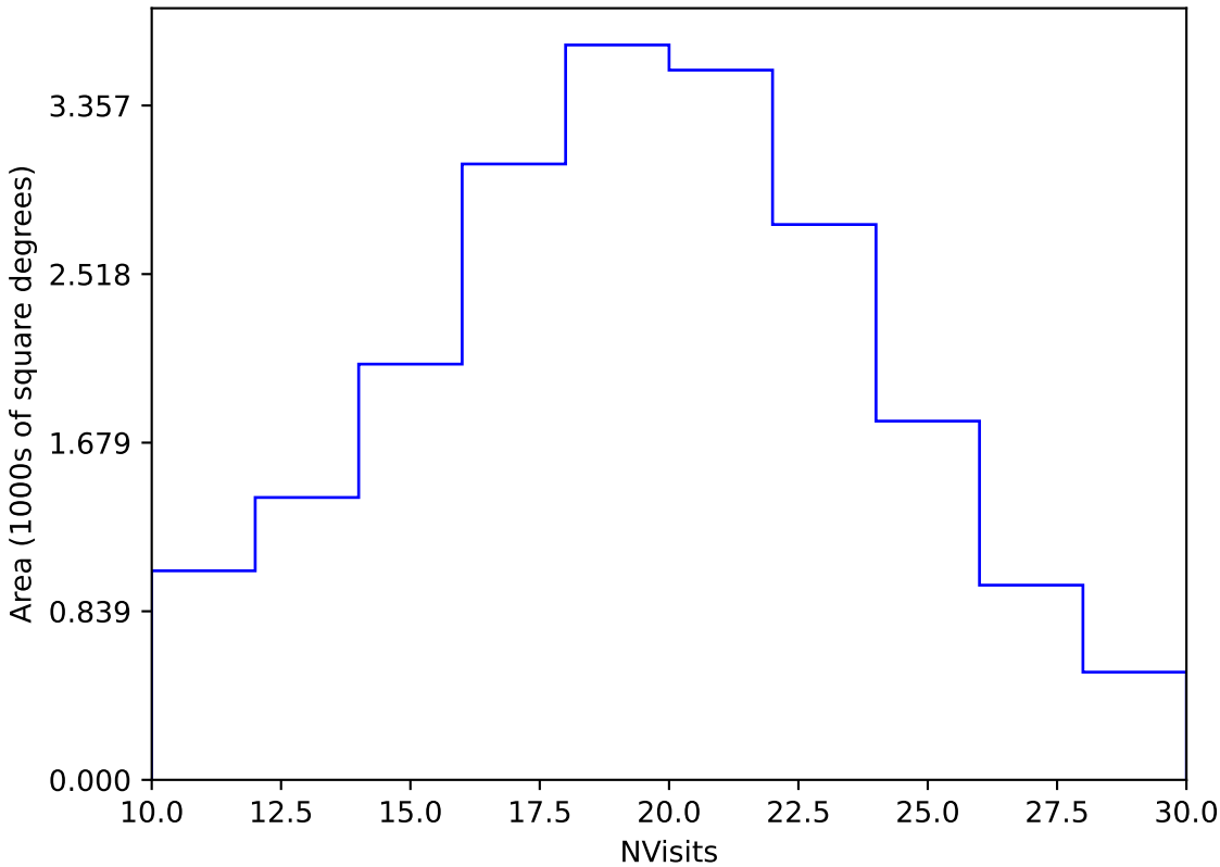
too_elab_heavy_r32_d3_ugrizy_v3.4_10yrs Yr 1 y band: NVisits
