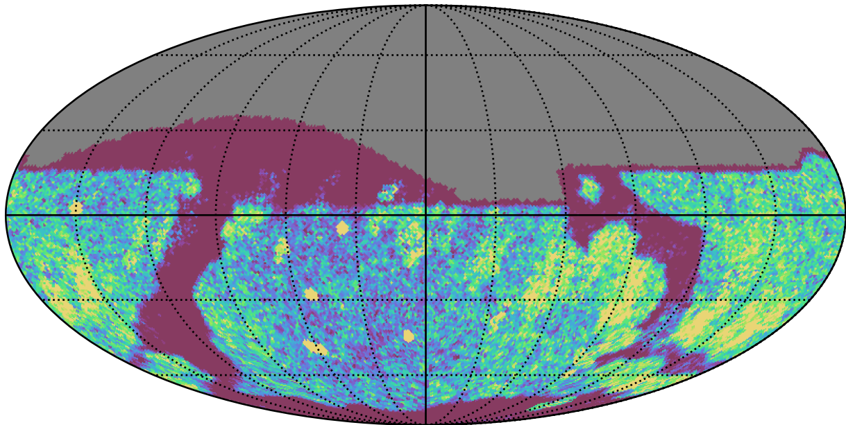
too_elab_heavy_r32_d3_ugrizy_v3.4_10yrs Yr 1 r band: NVisits
