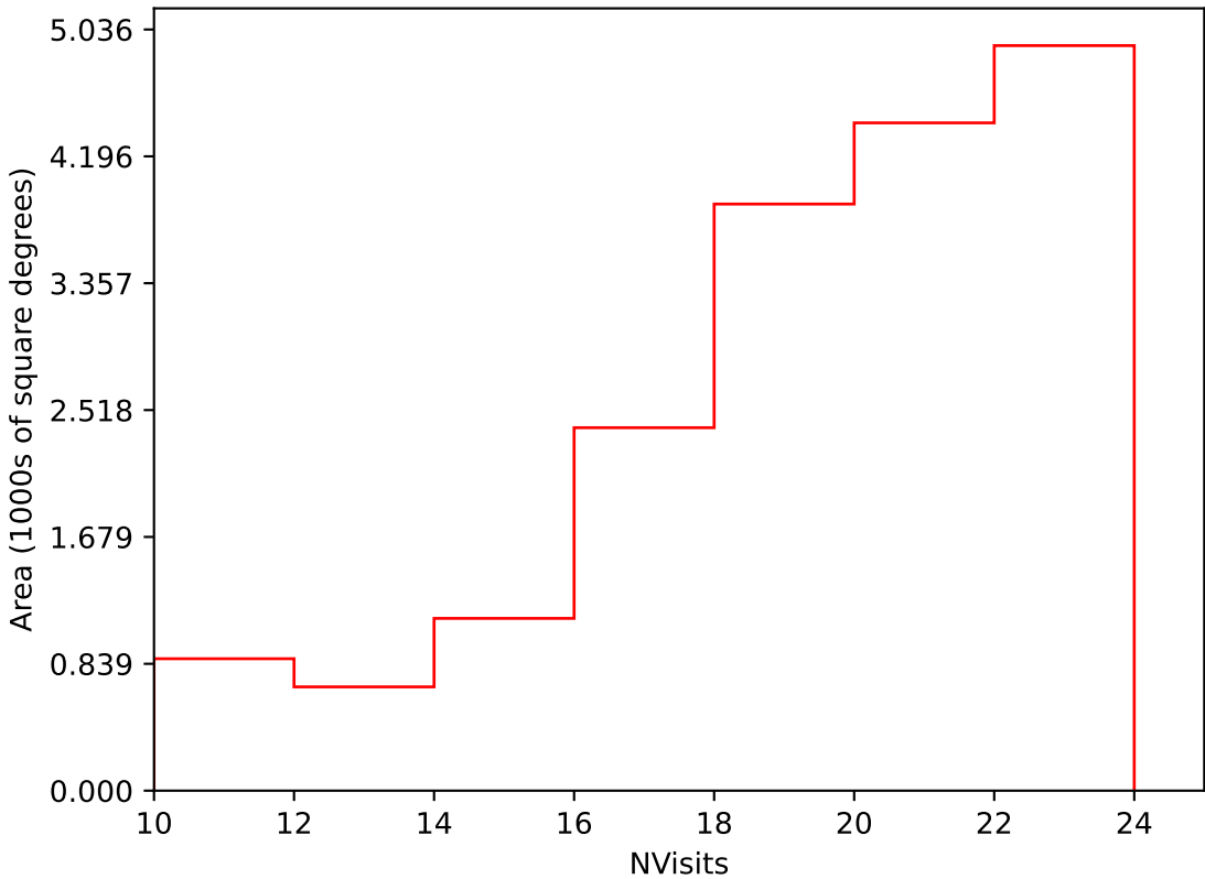
too_elab_heavy_r32_d3_ugrizy_v3.4_10yrs Yr 1 i band: NVisits
