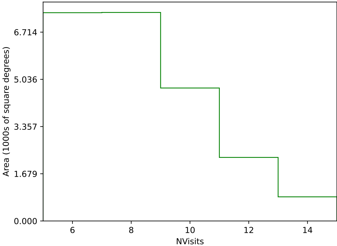
too_elab_heavy_r32_d3_ugrizy_v3.4_10yrs Yr 1 g band: NVisits
