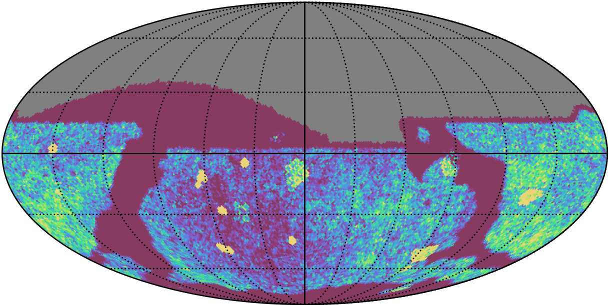
too_elab_heavy_r32_d3_ugrizy_v3.4_10yrs Yr 1 all bands: NVisits
